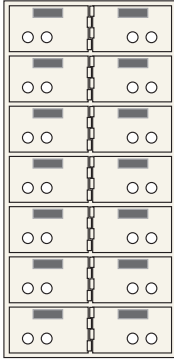
AXN-14 (Wt. 105 lbs.) 14 openings ea. 3" x 5"
