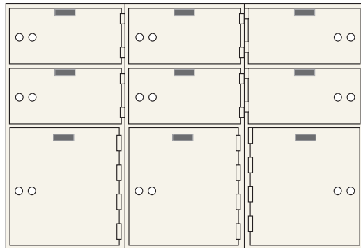
AX-9 (Wt. 195 lbs.) 6 openings ea. 5" x 10" 3 openings ea. 10" x 10"
