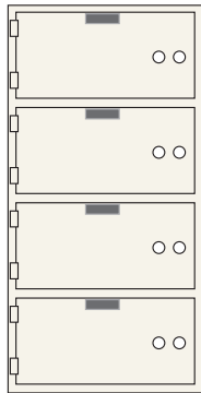
AXN-4 (Wt. 75 lbs.) 4 openings ea. 5" x 10"
