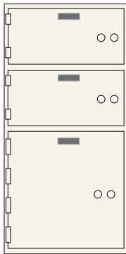
AXN-3 (Wt. 66 lbs.) 2 openings ea. 5" x 10" 1 opening ea. 10" x 10"
