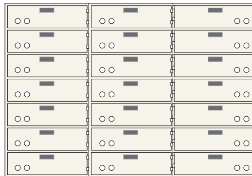
AX-21 (Wt. 260 lbs.) 21 openings ea. 3" x 10"
