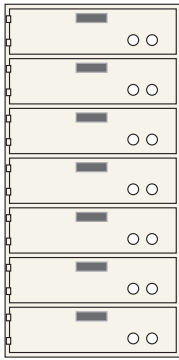
AXN-7 (Wt. 86 lbs.) 7 openings ea. 3" x 10"
